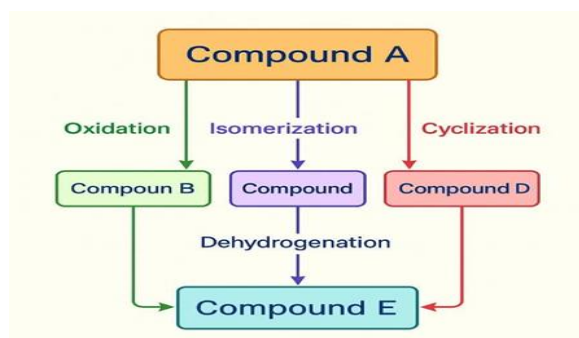
Fig. 1. Possible conversion reactions in essential oils.
