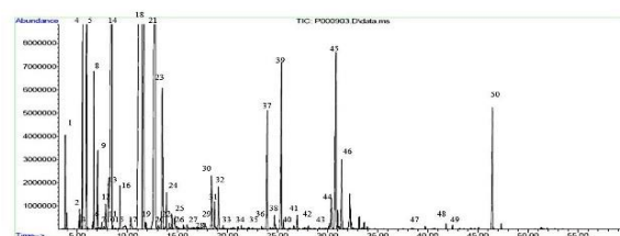
Fig. 6. GC/MS chromatograph of sage after distillation. Peak identification: 1. (Z)-Salvene; 2. Tricyclene; 3. \alpha -Thujene; 4. \alpha -Pinene; 5. Camphene; 6. Thuj-2,4(10)-diene; 7. Sabinene; 8. \beta -Pinene; 9. Myrcene; 10. \alpha -Phellandrene; 11. \alpha -Terpinene; 12. p -Cymene; 13. Limonene; 14. 1,8-Cineole; 15. (Z)- \beta -Ocimene; 16. g -Terpinene; 17. Terpinolene; 18. cis -Thujone; 19. trans -Thujone; 20. \alpha -Campholenal; 21. Camphor; 22. trans -Pinocamphone; 23. Borneol; 24. Terpinen-4-ol; 25. p -Cymen-8-ol; 26. \alpha -Terpineol; 27. Myrtenol; 28. trans -Carveol; 29. Unknown; 30. Bornyl acetate; 31. Thymol; 32. Carvacrol; 33. trans -Carvyl acetate; 34. \alpha -Terpinyl acetate; 35. Eugenol; 36. (Z)-Caryophyllene; 37. (E)-Caryophyllene; 38. Aromadendrene; 39. \alpha -Humulene; 40. allo-Aromadendrene; 41. Viridiflorene; 42. d -Cadinene; 43. Spathulenol; 44. Caryophyllene oxide; 45. Viridiflorol; 46. Humulene epoxide II; 47. 6,10,14-trimethyl-2-Pentadecanone; 48. Isopimara-9(11),15-diene; 49. Unknown; 50. Manool.
