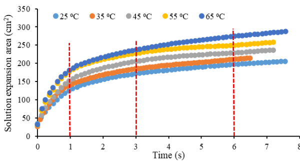
Fig. 9. Solution expansion area at different temperatures for 1.3% concentration.
