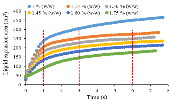
Fig. 10. Liquid expansion area of different concentration levels at 55 °C.
