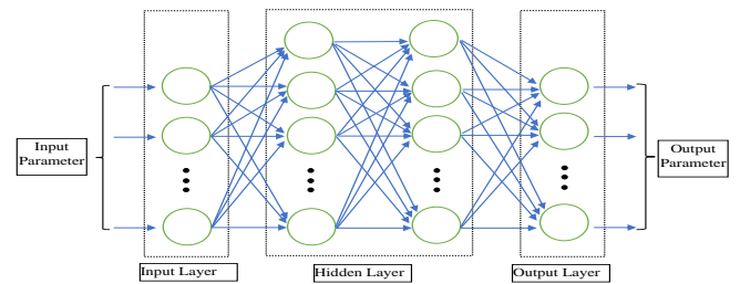
Fig. 5. Schematic representation of a multilayer perceptron ANN.
