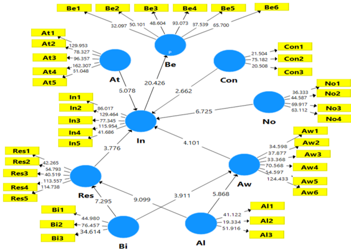
Fig. 4. Path model with t-values.
