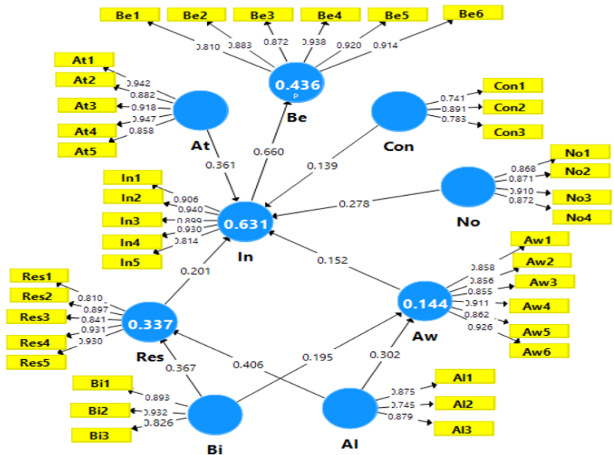
Fig. 3. Path model with standardized factor loadings.
