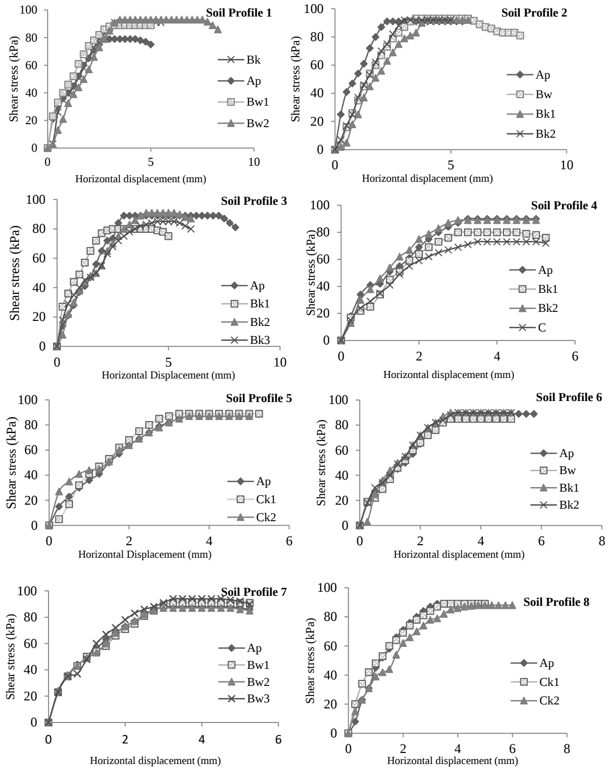
Fig. 5. The shear stress curves in terms of horizontal displacement against vertical stress in all soil profiles.
