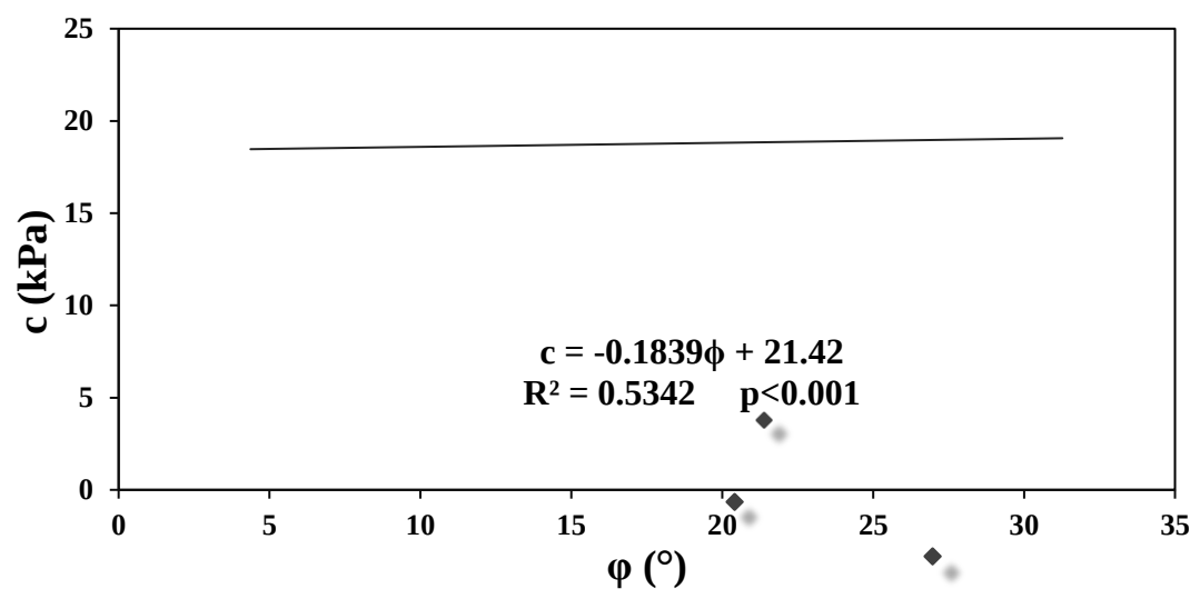
Fig. 3. The regression between soil cohesion (c, kPa) and the angle of internal friction ( \phi , °) the studied soils.
