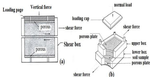
Fig. 2. Schematic diagram of the direct cutting test apparatus: (a) cross-section of the cutting box and (b) three-dimensional view of the direct cutting box with a square plan.
