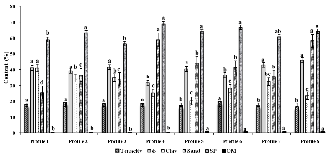
Fig. 4. Mean compression of some soil properties in different soil profiles. (φ: Internal friction angle; SP: Saturation percentage; OM: Organic matter).
