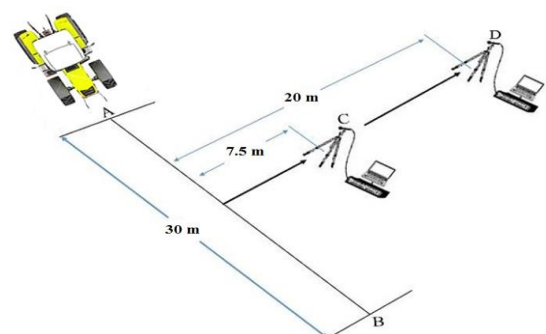
Fig. 3. Schematic of dimensions of measuring area of the noises emitted from tractors.
