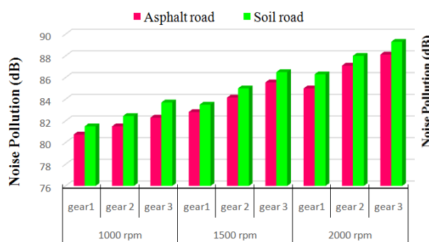
Fig. 5. Changes in sound pressure levels at the position of the driver's ear in different gears and engine speeds of New Holland tractor.
