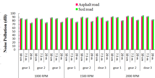
Fig. 6. The changes in sound pressure level at different distances of the microphone in the gear ratio and different speed of the John Deere tractor engine.
