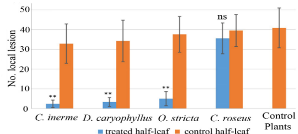
Fig. 3. The mean number of local lesions ( \pm standard deviation bars) resulting from the Tobacco mosaic virus inoculation of half-leaves of Nicotiana glutinosa alone (control half leaf), in comparison with the corresponding half-leaves pre-treated with aqueous extracts of various plant species (treated half-leaf). Control plants were inoculated only with Tobacco mosaic virus (TMV). **: significant difference at the 1% level between each treatment and its corresponding control. ns: not significant.
