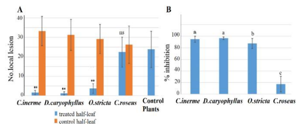
Fig. 2. (A) The mean number of local lesions per half leaves ( \pm standard deviation bars) and (B) percent of virus inhibition resulting from the inoculation of half-leaves of Nicotiana glutinosa with Tobacco mosaic virus alone (control half leaf), in comparison to the corresponding half-leaves treated with TMV mixed with aqueous extracts from four plant species (treated half-leaf). Different letters on columns (B) represent significant differences at P < 0.05 . **: significant difference at the 1% level between each treatment and its corresponding control. ns: not significant.
