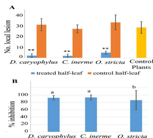
Fig. 6. (A) The mean number of local lesions ( \pm standard deviation bars) and (B) percent of virus inhibition resulting from the inoculation of half-leaves of Nicotiana glutinosa with Tobacco mosaic virus alone (control half leaf), in comparison to the corresponding half-leaves treated with TMV mixed with total protein extracts of various plant species (treated half-leaf). (B) Different letters on treatment bars represent significant differences at P < 0.05 . **: significant difference at the 1% level between each treatment and its corresponding control.
