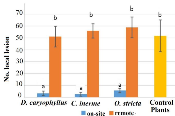
Fig. 7. Effects of total protein extracted from different plants species on systemic resistance induction against Tobacco mosaic virus infection in Nicotiana glutinosa . The assay involved application of total protein onto leaves of N. glutinosa , followed by inoculation with TMV, 24 h later, on these treated (on-site) as well as non-treated (remote) leaves. Data are presented as mean number of local lesions per leaf ( \pm standard deviation bars). Different letters on treatment bars represent significant differences at P < 0.05 .
