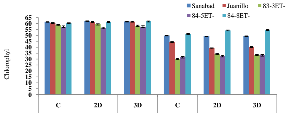
Fig. 1. Effect of moisture regimes and defoliation on flag leaf chlorophyll content (SPAD unit) of triticale cultivars at 10 days after anthesis (DAA). Control(c), defoliation of all leaves except the flag leaf (D2), and defoliation of all leaves except the flag leaf and penultimate leaf (D3). Vertical bars represent SE.
