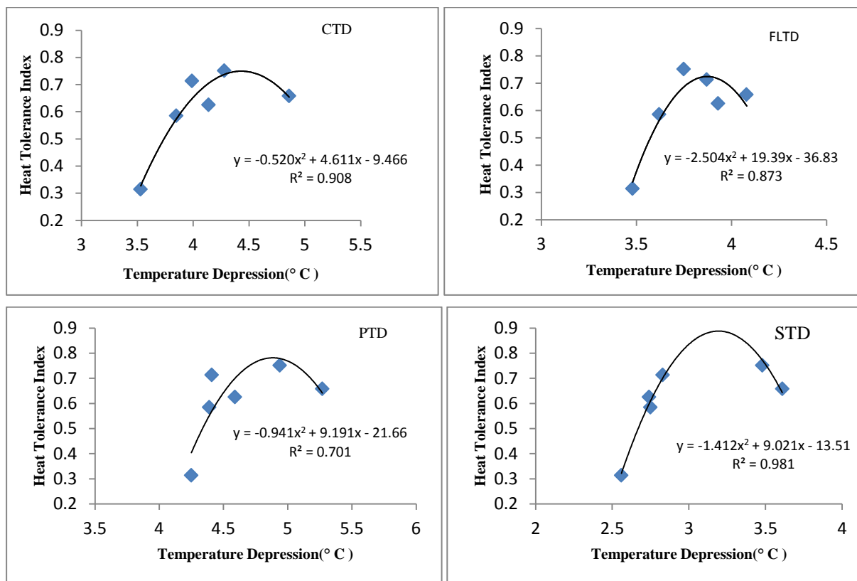
Fig. 4. Regression of PTD, STD, FLTD and CTD (°C) on Heat Tolerance Index; CTD: Canopy Temperature Depression; FLTD: Flag Leaf Temperature Depression; PTD: Peduncle Temperature Depression; STD: Spike Temperature Depression
