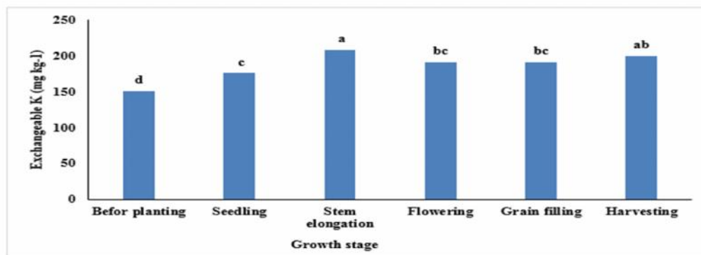
Fig. 2. Changes in contents of exchangeable K during different stages of rapeseed growth. Means followed by different letters are significantly different at P < 0.05 by Duncan's Multiple Range Test.
