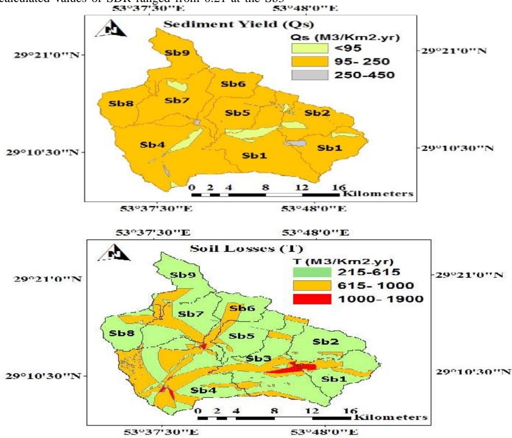
Fig. 2. A. Sediment yield B. Soil loss map of the Cachoyeh watershed based on the MPSIAC model
