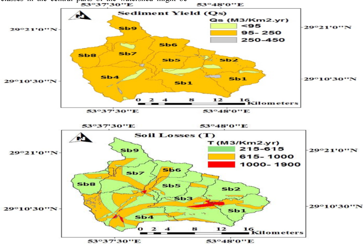
Fig. 2. A. Sediment yield B. Soil loss map of the Cachoyeh watershed based on the MPSIAC model
