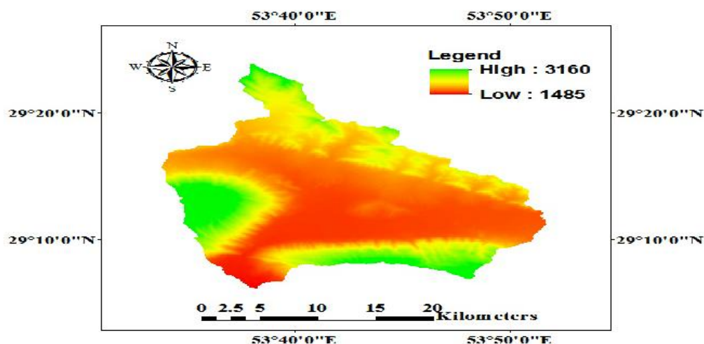
Fig.1. Location of the Cachoyeh watershed
